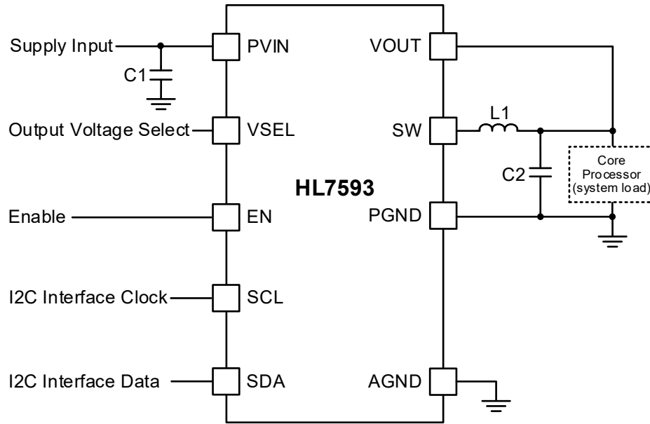
Figure 1. Typical Application Diagram
