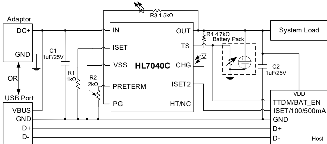
Figure 1. Typical Application Diagram
